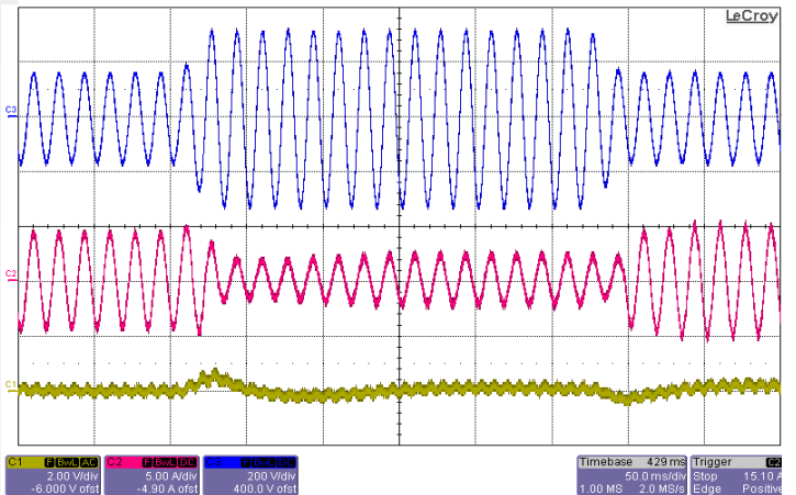
Figure 10: Input voltage transient response with 200 \mu F hold-up capacitor at full load current (115Vrms-230Vrms-115Vrms, 60Hz), Top: Vin (200V/div), Mid: Iin (5A/div), Bottom: Vout (2V/div), Timebase: (50ms/div).
