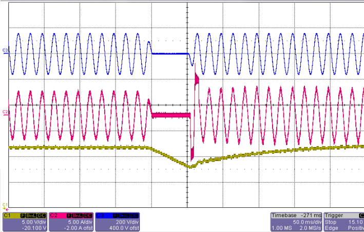
Figure 7: Line drop out with 400 \mu F hold-up capacitor at full load current (115Vrms, 60Hz) Top: Vin (200V/div), Mid: Iin (5A/div), Bottom: Vout (5V/div), Timebase: (50ms/div).
