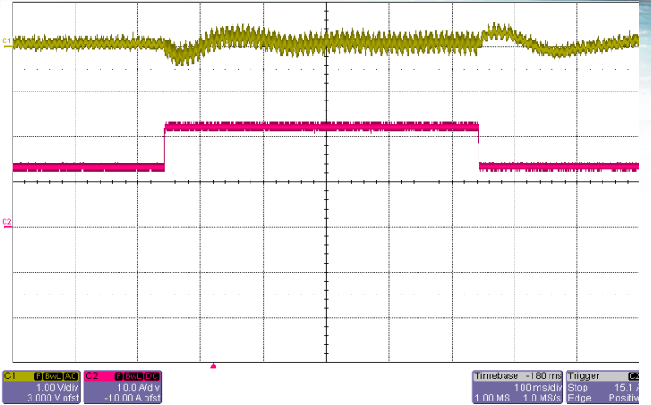
Figure 8: Output voltage response to step-change in load current with 200 \mu F hold-up capacitor (50%-75%-50% of Iout(max), 115Vrms, 60Hz) Top: Vout (1V/div), Bottom: Iout (10A/div), Timebase: (100ms/div).
